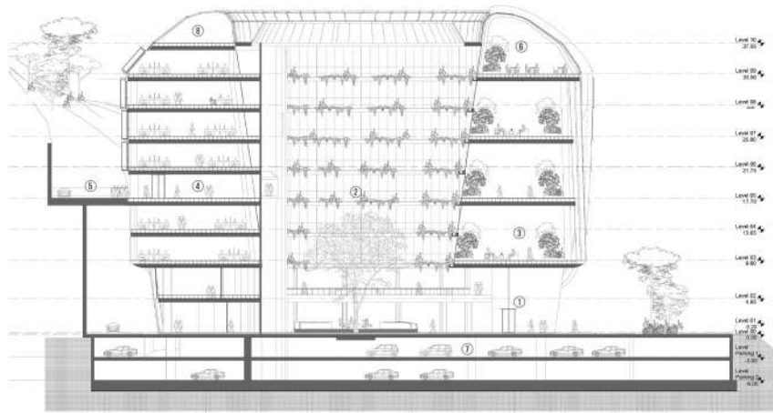
The section of the building
